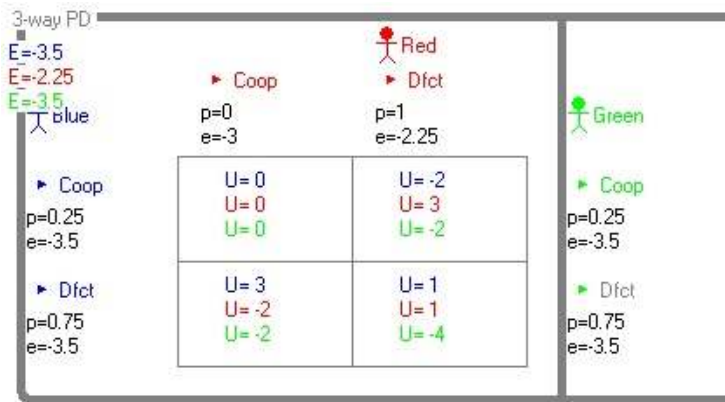
Figure 2.15: The Solution Window of a Normal Form Game
